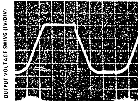
TIME (5 \mu\text{s/DIV} )
