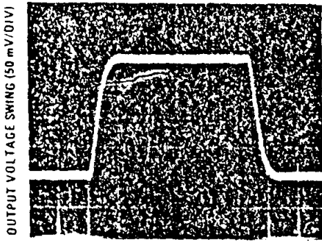
TIME (0.2 \mu\text{s/DIV} )
