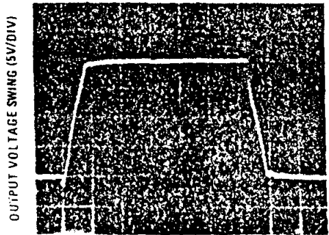
TIME (2 \mu\text{s/DIV} )
